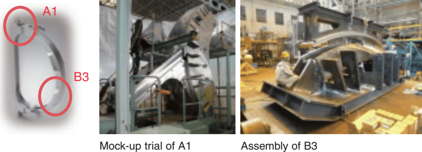
Fig.3-5 Full-scale segments of coil case
