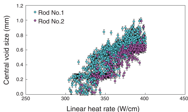
Fig.12-20 Formation of central void
