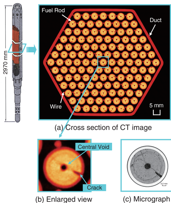
Fig.12-19 High-resolution computed tomography (CT) image of fuel assembly (upper) and enlarged view of fuel pellet (bottom)
