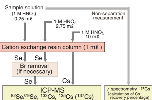
Fig.8-16 Analytical procedure for 79 Se and 135 Cs
