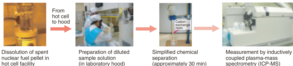
Fig.8-15 Procedure for determination of 79 Se and 135 Cs in spent nuclear fuel sample
