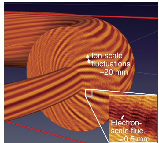
Fig.10-10 Electrostatic potential fluctuations in multi-scale fusion plasma turbulence
