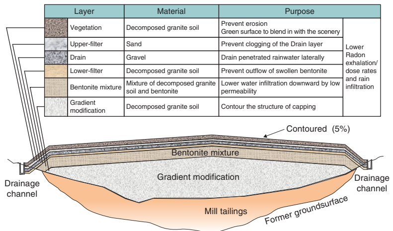
Fig.8-7 Structure and material of the capping constructed “Upstream”
