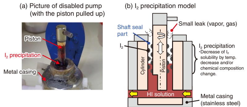
Fig.6-15 Pump malfunction during a hydrogen production test
