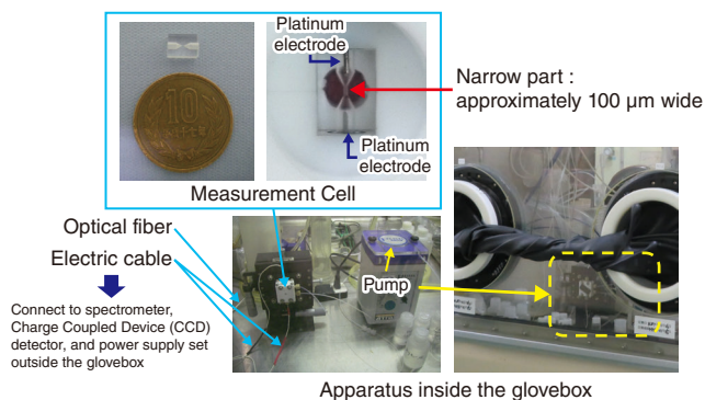
Fig.8-25 LEP-OES apparatus installed inside the glovebox
