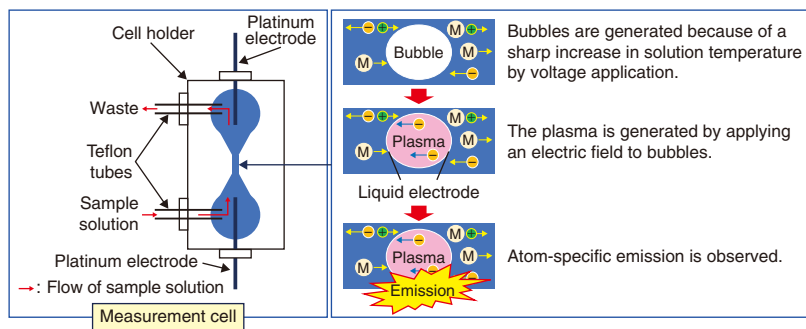
Fig.8-24 Liquid electrode plasma optical emission spectrometry (LEP-OES)
