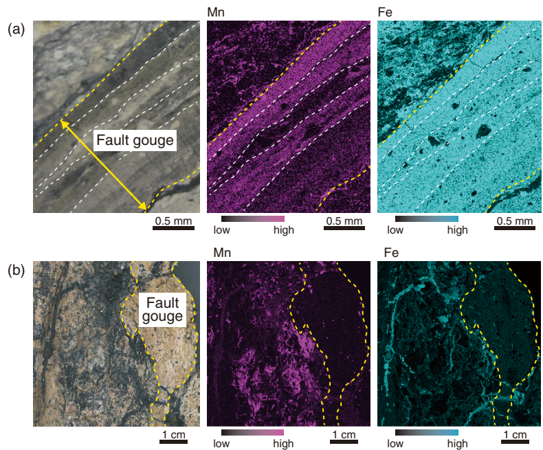
Fig.8-17 Photographs of polished sample surfaces and X-ray microscopy images showing spatial distribution of Mn and Fe from fault gouges of (a) capable and (b) incapable faults Mn and Fe are concentrated in the gouge of the capable fault.
