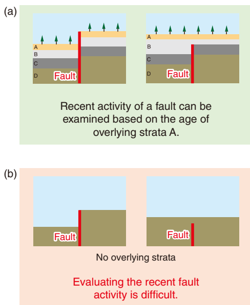
Fig.8-16 Identification of recent fault activity (a) with and (b) without overlying strata
